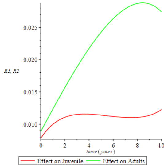
Figure 3.3 Recovery in the Juvenile sub-population when the probability of transmission is high in the adult sub-population ( \sigma_1 = 0.25 , \sigma_2 = 0.85 , \rho_1 = 0.150 , \rho_2 = 0.010 )
