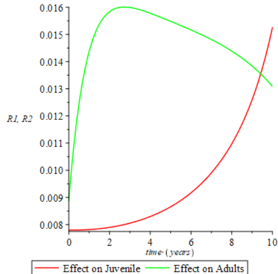
Figure 3.8 Recovery with high treatment rate when the probability of transmission is low and the juvenile sub-population is left untreated ( \sigma_1 = 0.00 , \sigma_2 = 0.85 , \rho_1 = 0.012 , \rho_2 = 0.35 ).
