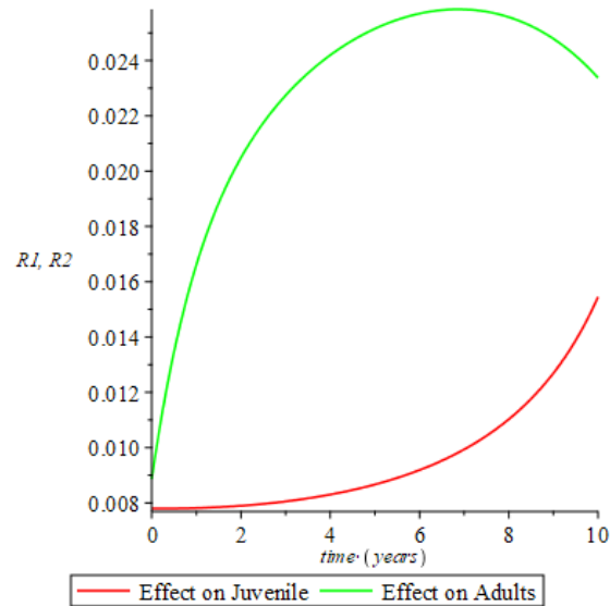
Figure 3.9 Recovery with high treatment rate when the probability of transmission is high and the juvenile sub-population is left untreated ( \sigma_1 = 0.00 , \sigma_2 = 0.85 , \beta = 0.150 , \beta' = 0.010 ).
