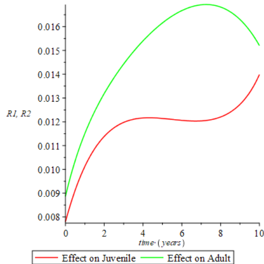
Figure 3.6 Recovery when the treatment rate is low and the probability of transmission is high and ( \sigma_1 = 0.25 , \sigma_2 = 0.25 , \rho_1 = 0.150 , \rho_2 = 0.010 ).
