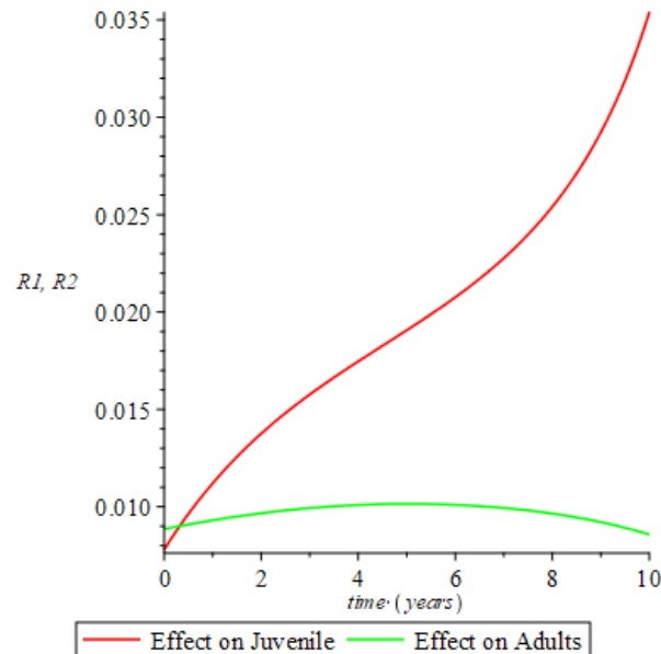
Figure 3.4 Recovery when the treatment rate is low and the probability of transmission is low ( \sigma_1 = 0.25 , \sigma_2 = 0.25 , \rho_1 = 0.012 , \rho_2 = 0.35 )
