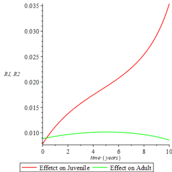
Figure 3.2 Recovery in the Adult sub-population when the probability of transmission is low in the adult sub-population ( \sigma_2 = 0.25 , \sigma_2 = 0.75 , \rho_1 = 0.012 , \rho_2 = 0.35 )
