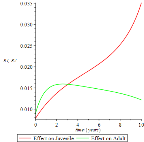
Figure 3.1 Recovery in the Juvenile sub-population when the probability of secondary transmission is low in the adult sub-population ( \sigma_1 = 0.25 , \sigma_1 = 0.85 , \rho_1 = 0.012 , \rho_2 = 0.35 ).
