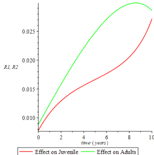
Figure 3.12 Recovery in the juvenile and adult sub-population when all newborns from infected mothers are HIV positive and treatment rate is low. ( \sigma_1 = 0.25 , \sigma_2 = 0.25 , \rho_1 = 0.075 , \rho_2 = 0.005 , \xi = 1.0 ).
