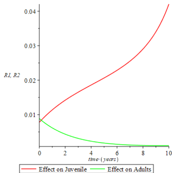
Figure 3.10 Recovery with low treatment rate when the probability of transmission is low and the adult sub-population is left untreated ( \sigma_1 = 0.25 , \sigma_2 = 0.00 , \rho_1 = 0.012 , \rho_2 = 0.35 )
