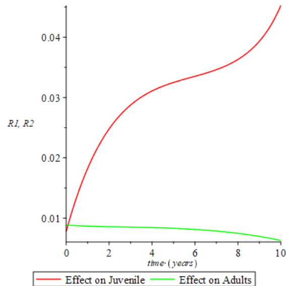
Figure 3.11 Recovery with high treatment rate when the probability of transmission is high and the adult sub-population is left untreated ( \sigma_1 = 0.85 , \sigma_2 = 0.00 , \rho_1 = 0.150 , \rho_2 = 0.010 ).
