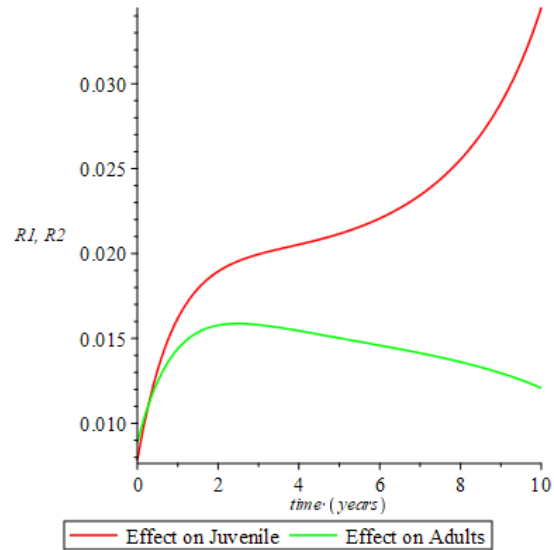
Figure 3.5 Recovery when the treatment rate is high and the probability of transmission is low ( \sigma_1 = 0.85 , \sigma_2 = 0.85 , \rho_1 = 0.012 , \rho_2 = 0.35 ).
