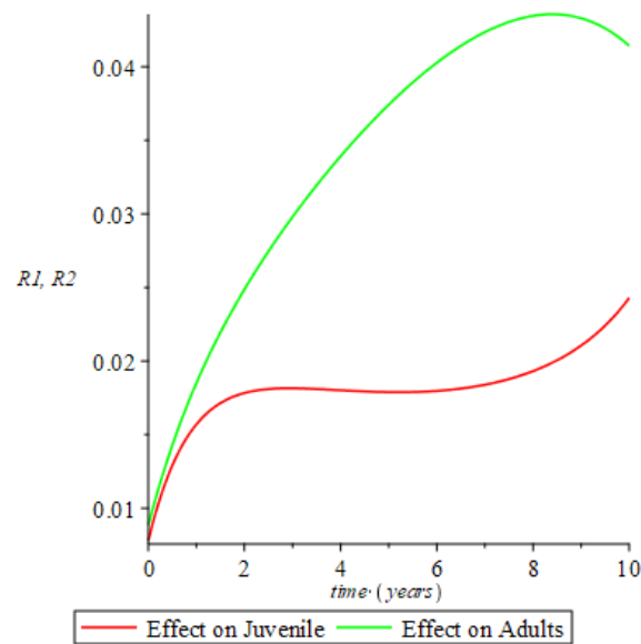
Figure 3.14 Recovery in the juvenile and adult sub-population when all newborns from infected mothers are HIV positive and treatment rate is high ( \sigma_1 = 0.85 , \sigma_2 = 0.85 , \rho_1 = 0.075 , \rho_2 = 0.005 , \xi = 1.0 ).
