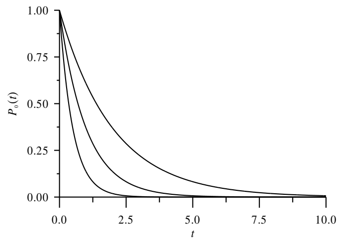
Fig. 1. Typical dependences of probability of freeing up of position of patient at increasing of quantity of requests of service
